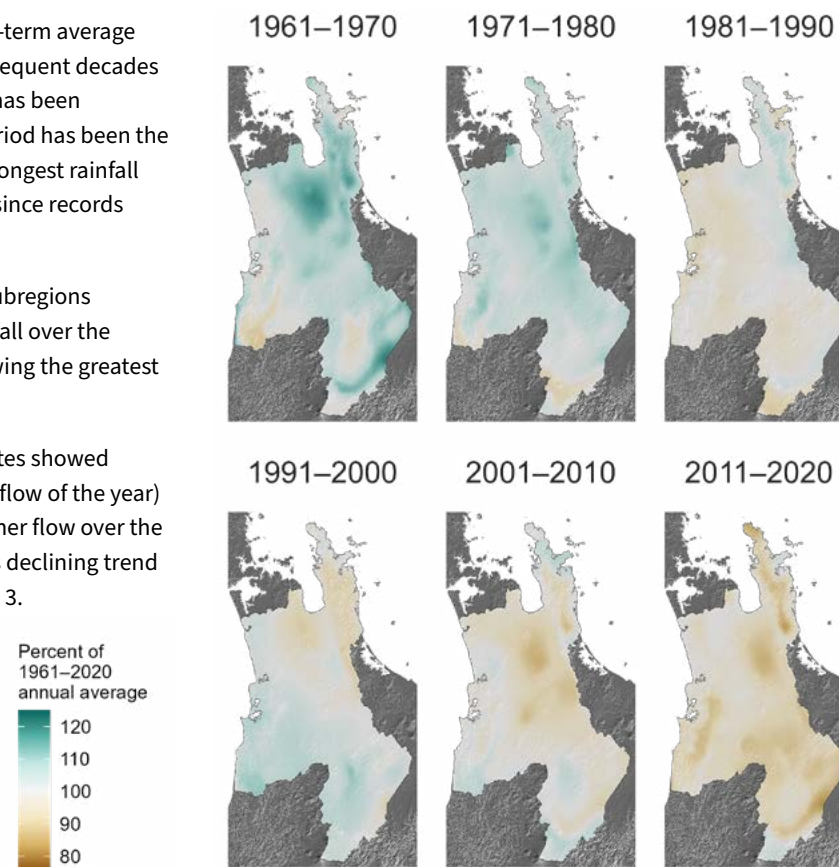
Figure 2: Waikato region decadal rainfall as a percent of the long-term rainfall (1961-2020) using NIWA's Virtual Climate Station dataset.
