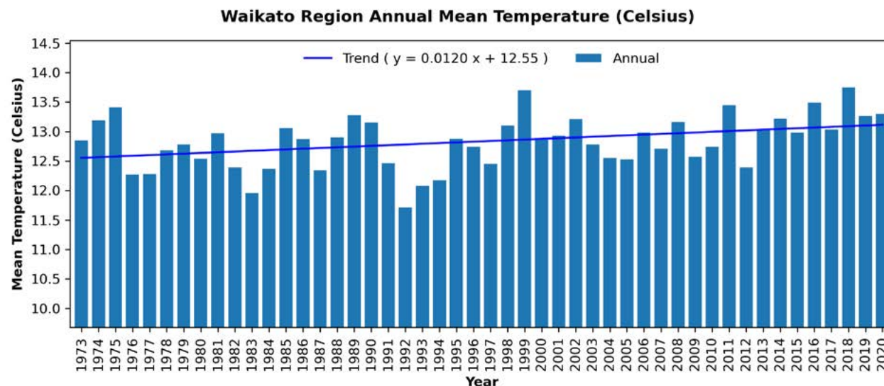
Figure 1: Long-term pattern in annual mean temperature across Waikato region.
